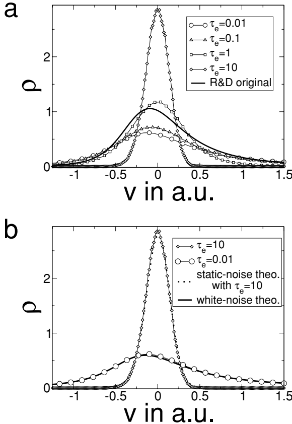
Figure 1: Probability density of the shifted voltage compared to results of numerical simulations. (a) Density according to equation 2.12 (theory by R&D) is compared to simulations at different correlation times as indicated ( \tau_i = 5\tau_e ). Since the noise intensities are fixed, the simulated densities at different \tau_e should all fall onto the solid line according to equation 2.12, which is not the case. (b) The simulations at small ( \tau_e = 0.01 ) and large ( \tau_e = 10 ) correlation times are compared to our expressions found in the limit case of white and static noise: equations 3.8 and 5.4, respectively. Note that in the constant-intensity scaling, equation 5.4 depends implicitly on \tau_{e,i} since the variances change as \sigma_{e,i} = Q_{e,i}/\tau_{e,i} . Parameters: \beta = 1 , Q_e = 0.075 , Q_i = 0.75 , Q_I = 0 , \Delta t = 0.001 , and simulation time T = 10^5 .
