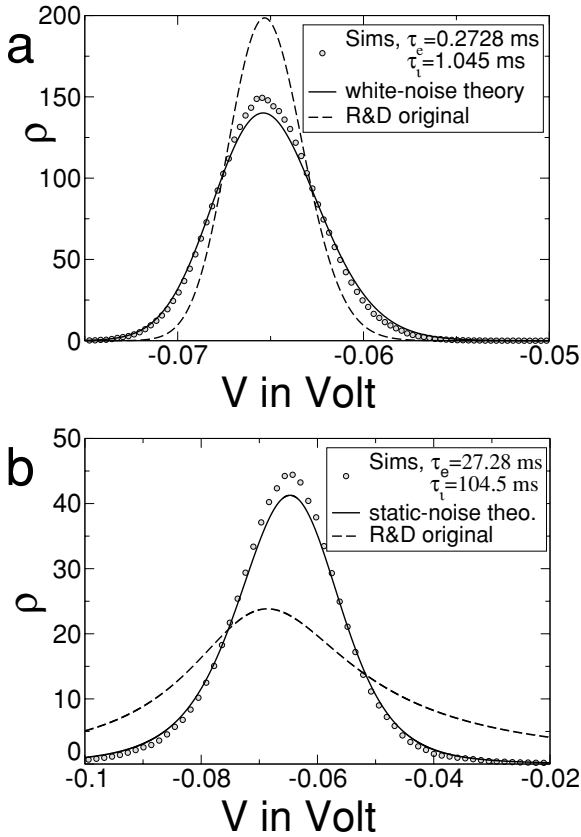
Figure 3: Probability density of membrane voltage for different orders of magnitude of the correlation times \tau_e , \tau_i . Parameters as in Figure 2 except for the correlation times, which were chosen one order of magnitude smaller (a) or larger (b).
