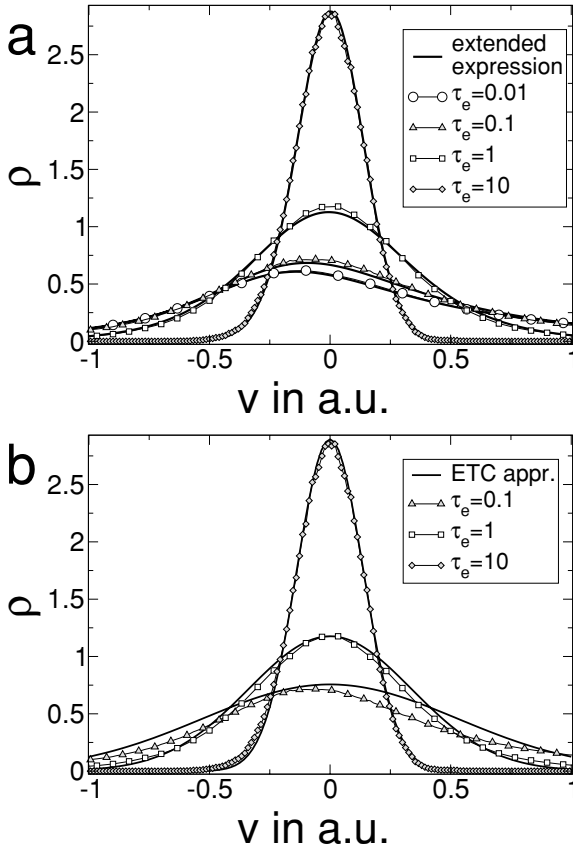
Figure 4: Probability density of membrane voltage for simulation data and parameters as in Figure 1a. The extended expression equation 2.15 (a) and the effective time constant approximation, equation 2.25 (b), are compared to results of numerical simulations.
