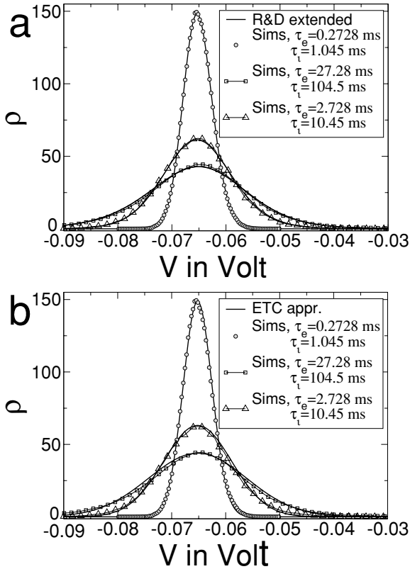
Figure 5: Probability density of membrane voltage for simulation data and parameters as in Figures 2 and 3. The extended expression, equation 2.15 (a), and the effective time constant approximation, equation 2.25 (b), are compared to results of numerical simulations.
