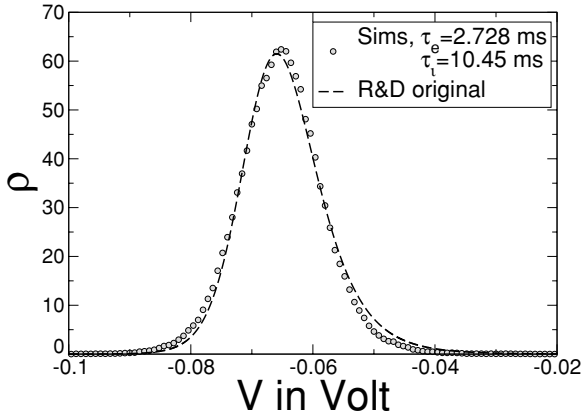
Figure 2: Probability density of membrane voltage corresponding to the parameters in Figure 2b of Rudolph and Destexhe (2003): g_L = 0.0452 \text{ mS/cm}^2 , a = 34636 \text{ } \mu\text{m}^2 , C_m = 1 \text{ } \mu\text{F/cm}^2 , E_L = -80 \text{ mV} , E_e = 0 \text{ mV} , E_i = -75 \text{ mV} , \sigma_e = 0.012 \text{ } \mu\text{S} , \sigma_i = 0.0264 \text{ } \mu\text{S} , g_{e0} = 0.0121 \text{ } \mu\text{S} , g_{i0} = 0.0573 \text{ } \mu\text{S} ; additive-noise parameters ( \sigma_I, I_0 ) are all zero; we used a time step of \Delta t = 0.1 \text{ ms} and a simulation time of 100 s.
