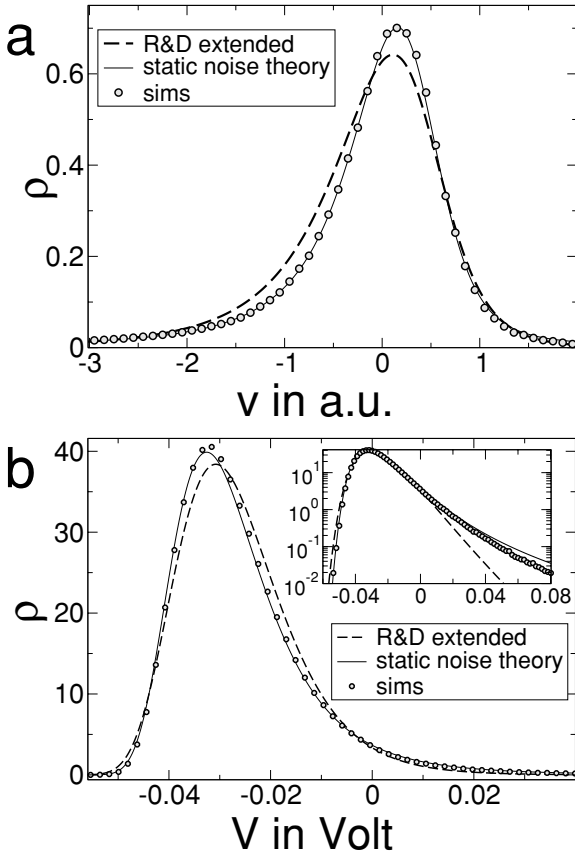
Figure 6: Probability density of membrane voltage for long correlation times; static noise theory, (equation 5.4, solid lines) and extended expression by R&D (equation 2.15, dashed lines) against numerical simulations (symbols). (a) Density of the shifted variable v with Q_e = Q_i = 3 , \beta = 1 , \tau_e = \tau_i = 20 , V_e = 1.5 , V_i = -0.5 . Here, the mean value is infinite. In the simulation, we implemented reflecting boundaries affecting the density only in its tails (not shown in the figure). (b) Density for the original voltage variable with g_L = 0.0452 mS/cm 2 , a = 34 , 636 \mu\text{m}^2 , C_m = 1 \mu\text{F}/\text{cm}^2 , E_L = -80 mV, E_e = 0 mV, E_i = -75 mV, \sigma_e = 0.012 \mu\text{S} , \sigma_i = 0.045 \mu\text{S} , g_{e0} = 0.121 \mu\text{S} , g_{i0} = 0.0574 \mu\text{S} , \tau_e = 7.5 ms, \tau_i = 30 ms. Here the mean value is finite. Inset: Same data on a logarithmic scale.
