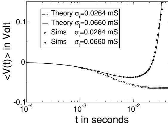
Figure 8: Time-dependent mean value of the original voltage variable (in volts) as a function of time (in seconds) for the initial value V(t=0) = 0 V and different values of the inhibitory conductance standard deviation \sigma_i ; numerical simulations of equations 2.19 and 2.20 (circles) and theory according to equation 6.3 (solid lines). For all curves, g_{e0} = 0.0121 \mu\text{S} , g_{i0} = 0.0573 \mu\text{S} , \sigma_e = 0.012 \mu\text{S} , \tau_e = 2.728 ms, \tau_i = 10.49 ms, a = 34.636 \mu\text{m}^2 , and C_m = 1 \mu\text{F}/\text{cm}^2 . For the dashed line (theory) and the gray squares (simulations), we choose \sigma_i = 0.0264 \mu\text{S} ; hence, in this case, parameters correspond to the standard parameter set by Rudolph and Destexhe (2003). For the solid line (theory) and the black circles, we used \sigma_i = 0.066 \mu\text{S} corresponding to the 250% of the standard value by R&D. At the standard parameter set, the mean value saturates at a finite level, in the second case, the mean diverges and goes beyond 100 mV within 31 ms. Simulations were carried out for 10^6 voltage trajectories using an adaptive time step (always smaller than 0.01 ms) that properly took into account the trajectories that diverge the strongest. The large number of trajectories was required in order to get a reliable estimate of the time-dependent mean value in the case of strong noise ( \sigma_i = 0.066 \mu\text{S} ) where voltage fluctuations are quite large.
