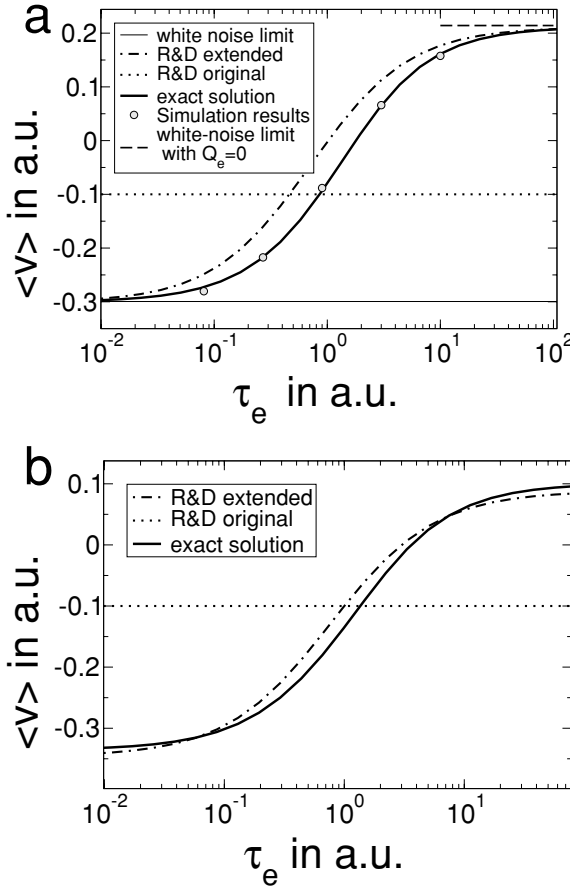
Figure 7: Stationary mean value of the shifted voltage (in arbitrary units) versus correlation time (in arbitrary units) of the excitatory conductance. Noise intensities Q_e = 0.2 , Q_i = 0.3 , Q_l = 0 , and \beta = 1 are fixed in all panels. Correlation time of the inhibitory conductance: \tau_i = 10^{-2} (a) and \tau_i = 1 (b). Shown are the exact analytical result, equation 6.7 (solid line); the mean value according to the original solution, equation 6.9 (dotted line); and the mean value according to the extended expression, equation 6.10 (dash-dotted line). In panel a , we also compare to the mean value of the white noise solution for Q_e = 0.2 , Q_i = 0.3 (thin solid line) and for Q_e = 0 , Q_i = 0.3 (dashed line), as well as to numerical simulation results (symbols).
